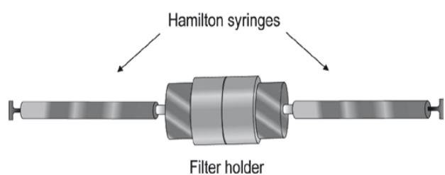
Figure 3. Extruder.
